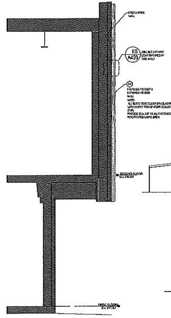
A5 EXT WALL SECTION AT EAST WING A.300 SCALE: 1/2" = 1'-0"
